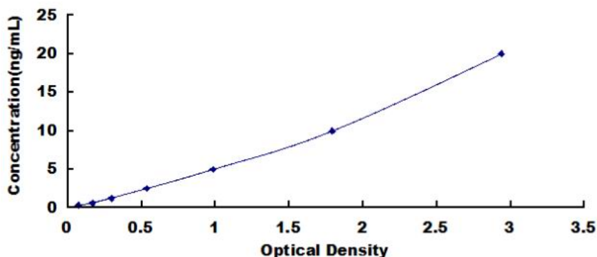
Typical Standard Curve for Human ANGPTL2 ELISA.
