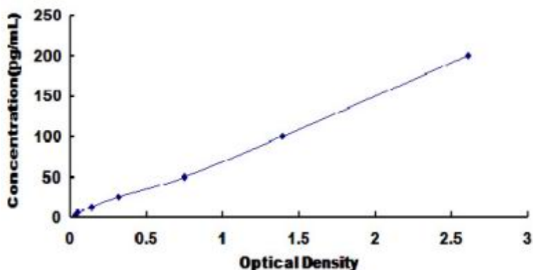
Typical Standard Curve for Rat ANGPT1 ELISA.
