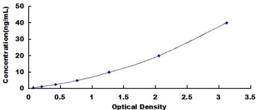
Typical Standard Curve for Rat ALDOC ELISA.
