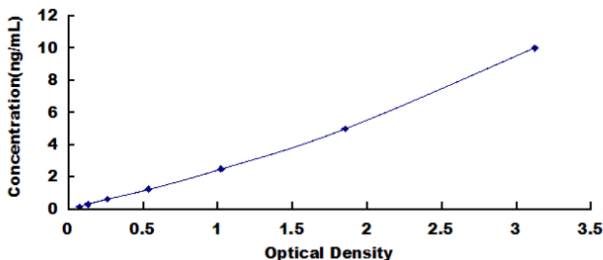
Typical Standard Curve for Mouse AGR2 ELISA.
