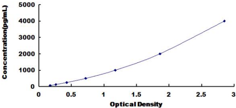
Typical Standard Curve for Human ADAMTS4 ELISA.
