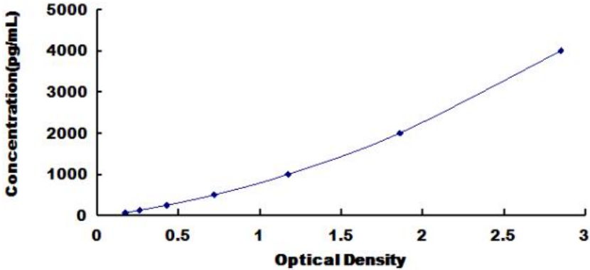
Typical Standard Curve for Mouse ACE2 ELISA.
