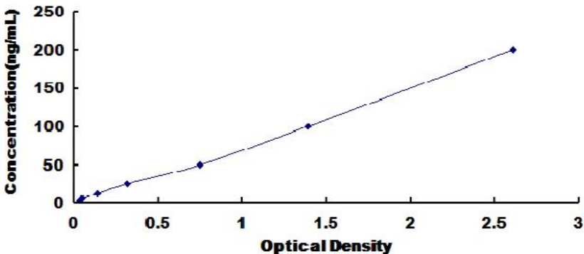
Typical Standard Curve for Rat ACE ELISA.
