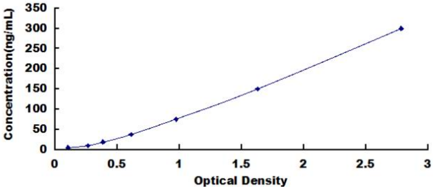
Typical Standard Curve for Human aZGP1 ELISA.
