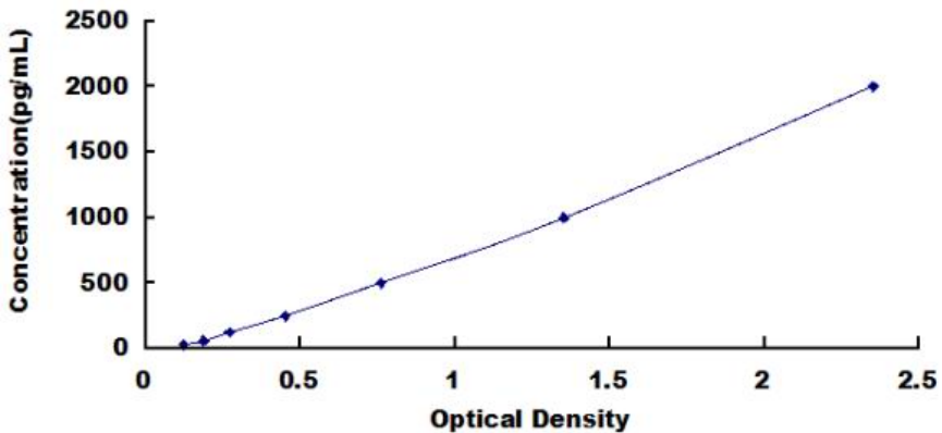
Typical Standard Curve for Bovine VEGF165 ELISA.
