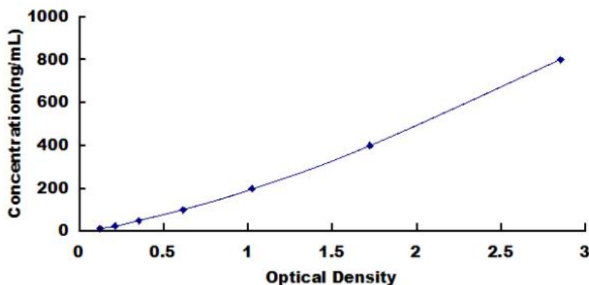
Typical Standard Curve for Equine Ub ELISA.
