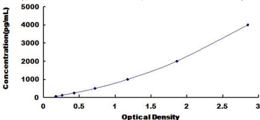
Typical Standard Curve for Mouse TremI2 ELISA.
