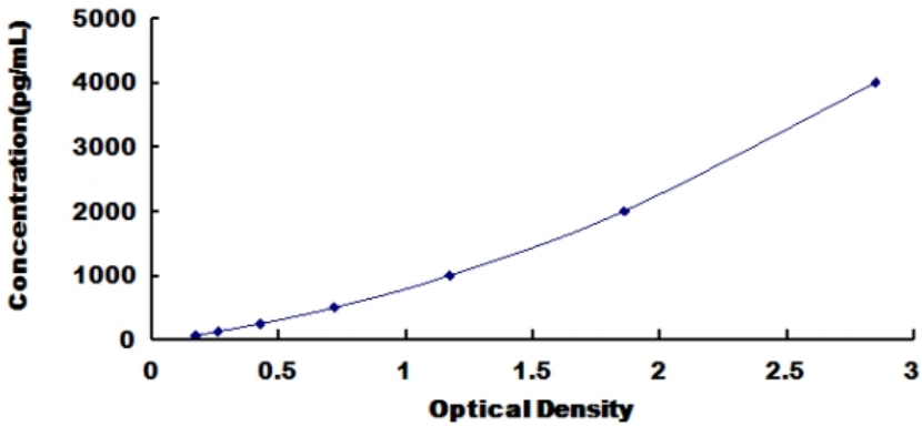
Typical Standard Curve for Mouse TSH ELISA.
