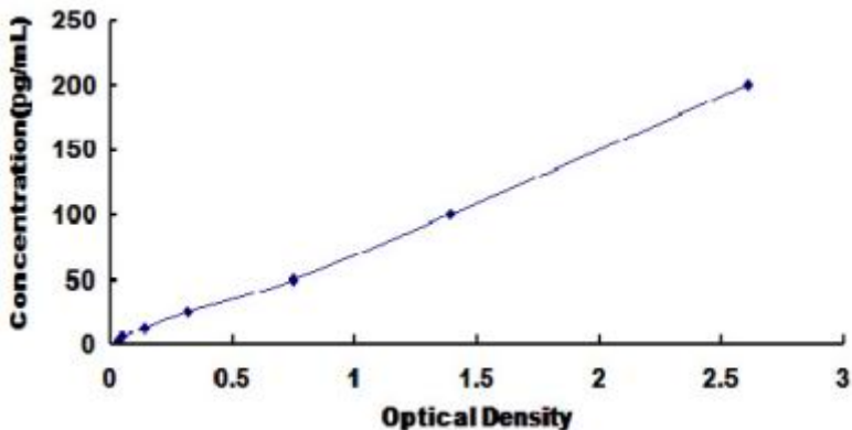
Typical Standard Curve for Canine TNFa ELISA.
