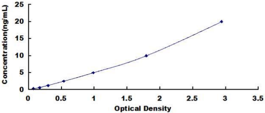
Typical Standard Curve for Mouse SIRT7 ELISA.
