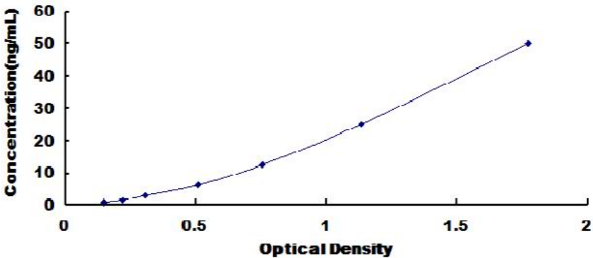
Typical Standard Curve for Bovine PF4 ELISA.
