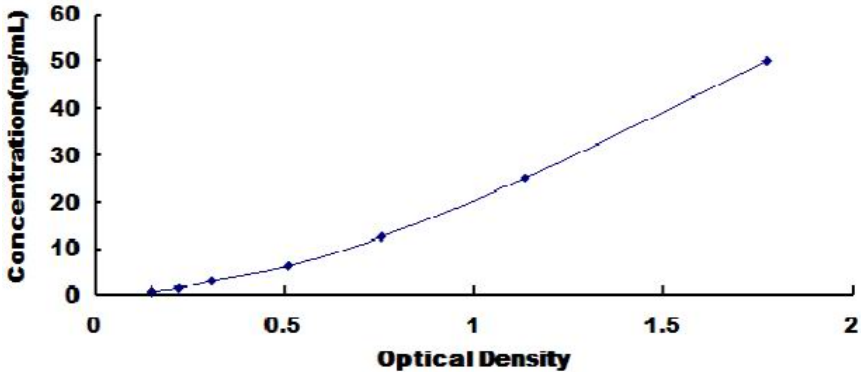
Typical Standard Curve for Human NRG4 ELISA.
