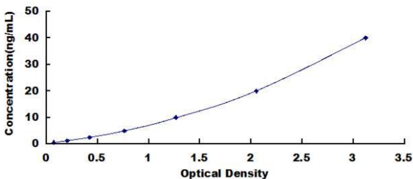
Typical Standard Curve for Human ITM2B ELISA.
