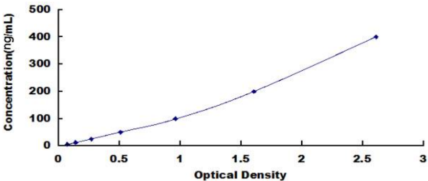
Typical Standard Curve for Mouse IGFBP6 ELISA.
