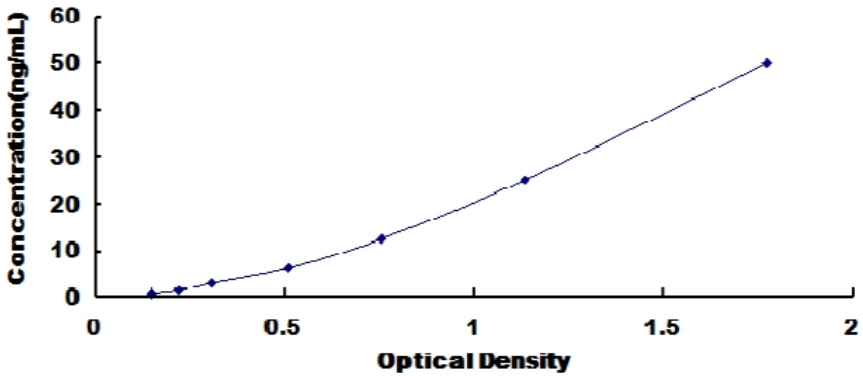
Typical Standard Curve for Bovine FSH ELISA.
