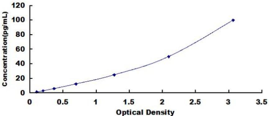
Typical Standard Curve for Human FGF21 ELISA.
