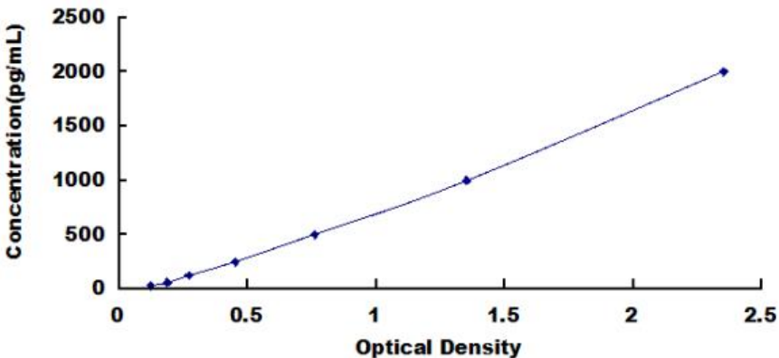
Typical Standard Curve for Mouse FGF15 ELISA.
