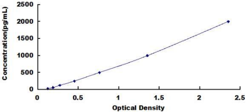
Typical Standard Curve for Human CWF19L2 ELISA.
