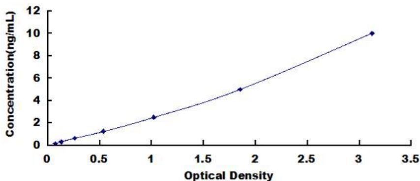
Typical Standard Curve for Human CRLF2 ELISA.
