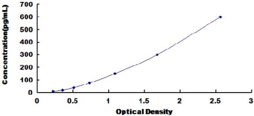
Typical Standard Curve for Rat CALB ELISA.
