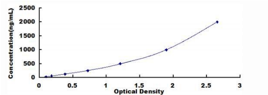
Typical Standard Curve for Rat ADP ELISA.
